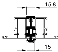
FT-0121/A kg/m 0.669
