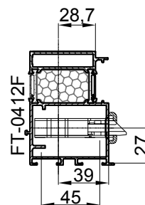
Obrada krila za bravu 45 (MR2) Processing of sash for multipoint lock with massive bolt 45 (MR2)
