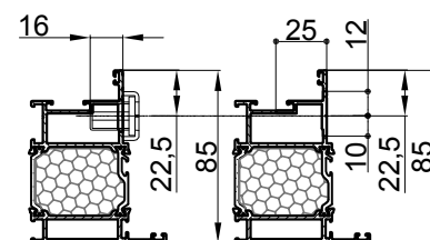
Obrada rama za prihvatne pločice FT-0402F Processing of frame for striking plate
