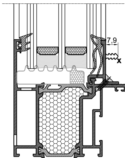
B-B FT-0400F
