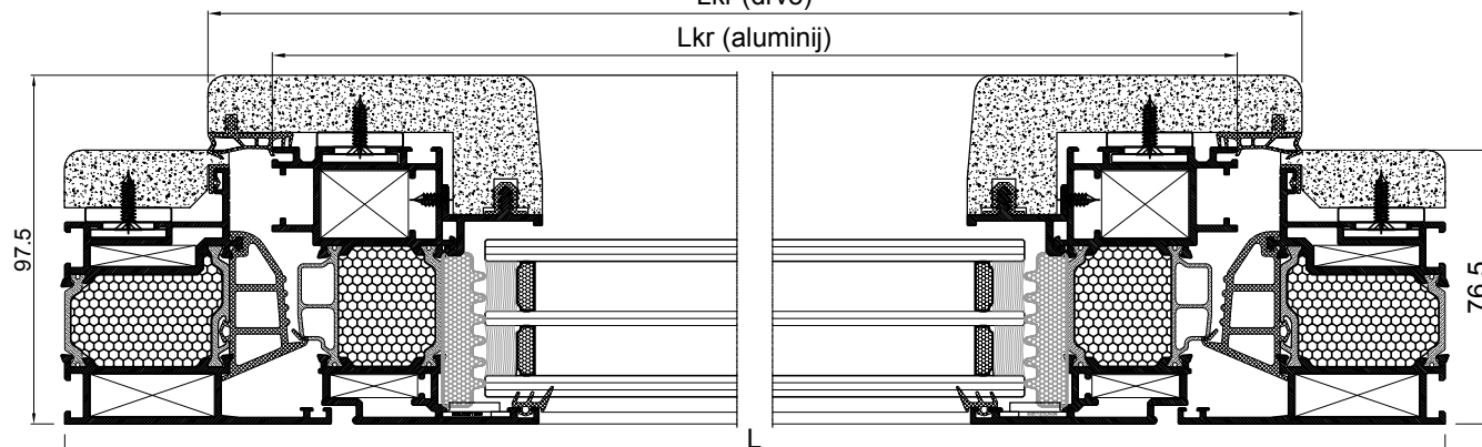
Staklo Glass
