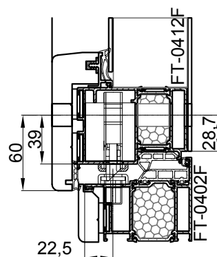
Obrada krila za bravu 45 (MR2) Processing of sash for multipoint lock with massive bolt 45 (MR2)
