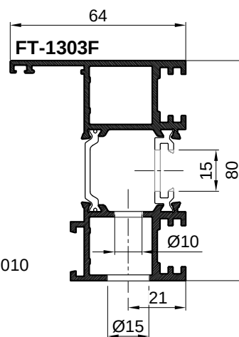
PRESJEK 2-2 SECTION 2-2
