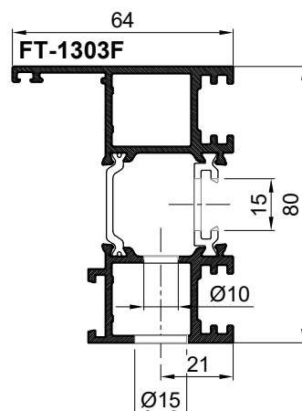
PRESJEK 2-2 SECTION 2-2
