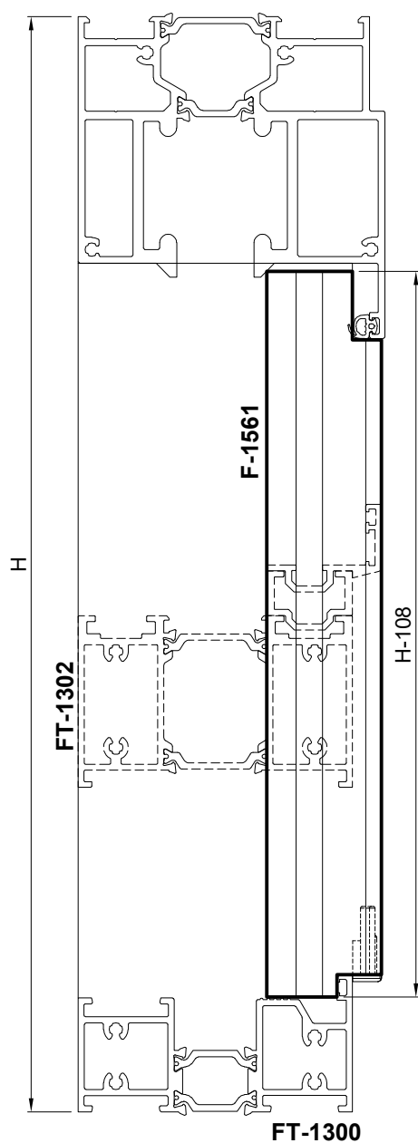
PRESJEK 1-1 SECTION 1-1
