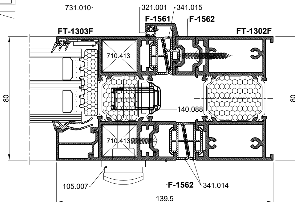
PRESJEK 4 CROSS SECTION 4
