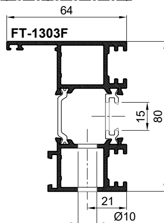
PRESJEK 1-1 SECTION 1-1
