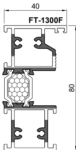
OBRADA PROFILA FT-1300F i FT-1304F PROCESSING PROFILE FT-1300F and FT-1304F
