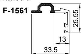
PRESJEK 2-2 SECTION 2-2
