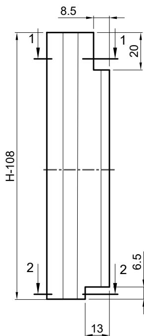
PRESJEK 1-1 SECTION 1-1
