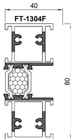
OBRADA PROFILA FT-1300F i FT-1304F PROCESSING PROFILE FT-1300F and FT-1304F
