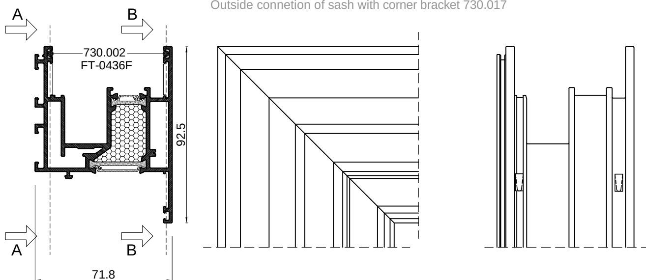
Spajanje kutnikom 730.017 Connecting with cor. brac. 730.017
