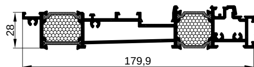
FT-0433F kg/m 3.0646
