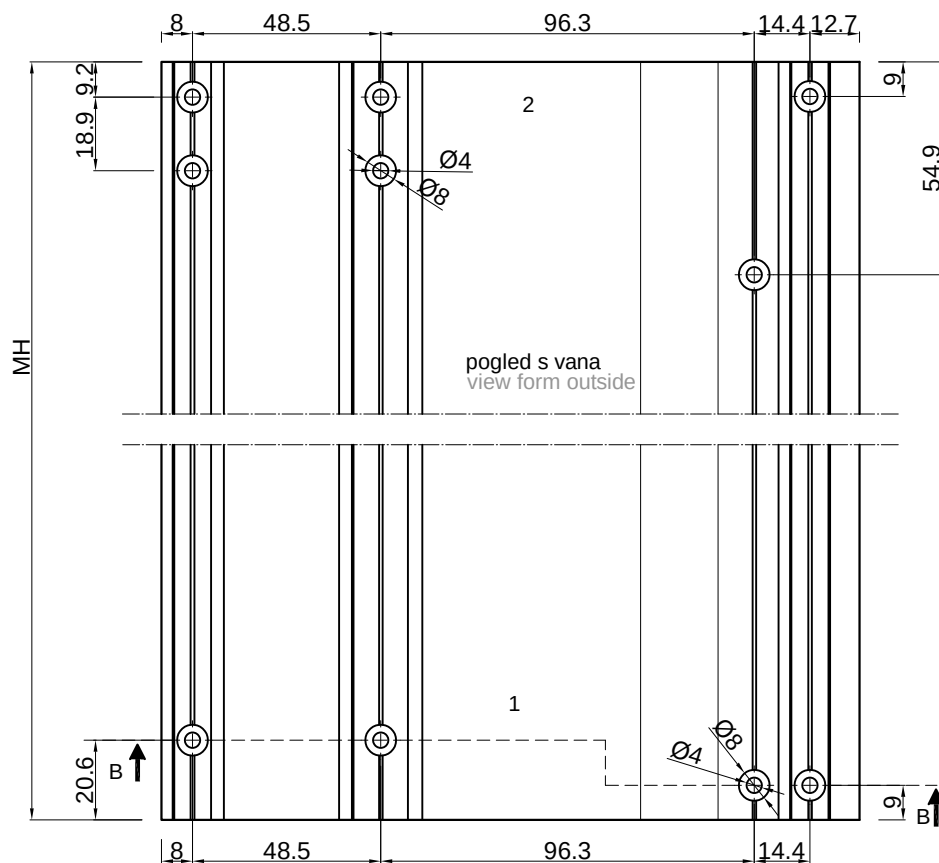
presjek B-B M 1.5:1 cross section B-B M 1.5:1
