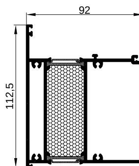
FT-0442F kg/m 2.977
