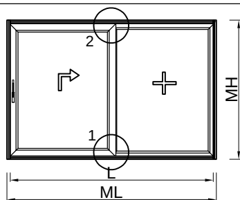
detalj 2 detail 2
