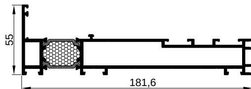
FT-0431F kg/m 2.778
