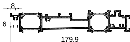
M 2:1 presjek C-C M 2:1 cross section C-C
