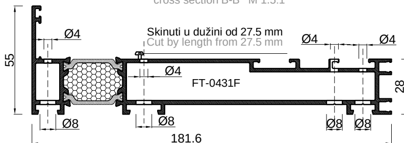
presjek B-B M 1.5:1 cross section B-B M 1.5:1
