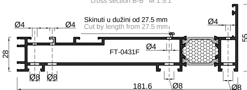
presjek B-B M 1.5:1 cross section B-B M 1.5:1
