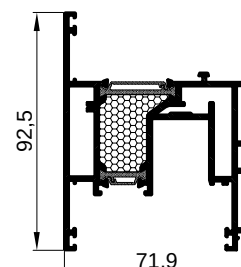
FT-0436F kg/m 2.396
