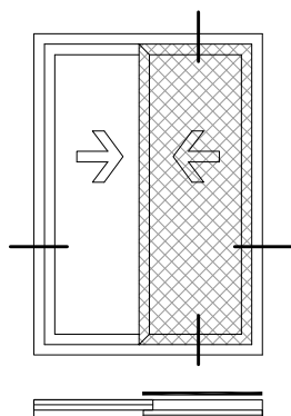
DETALJ S KLIZNOM KOMARICOM DETAIL WITH SLIDING MOSQUITO NET
